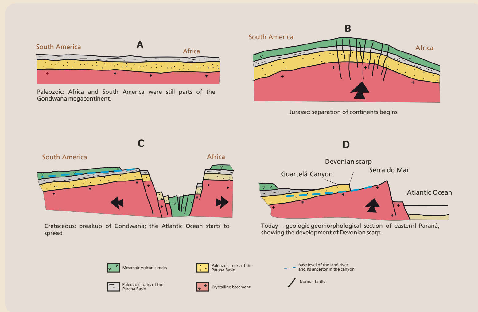
Coastal evolution of Paraná showing the continental breakup, the Guartelá Canyon carving, and the sculpturing of the Devonian scarp.
