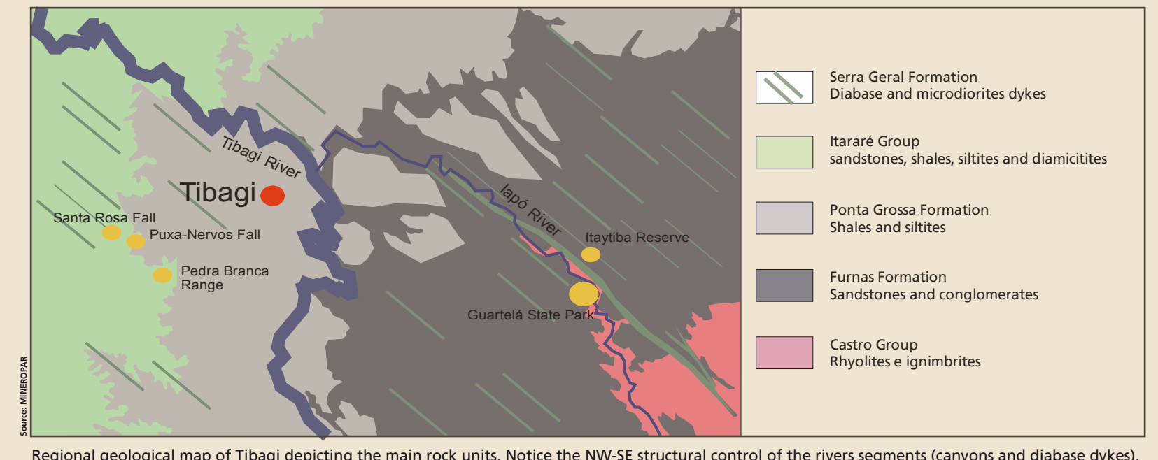
Regional geological map of Tibagi depicting the main rock units. Notice the NW-SE structural control of the rivers segments (canyons and diabase dykes).
