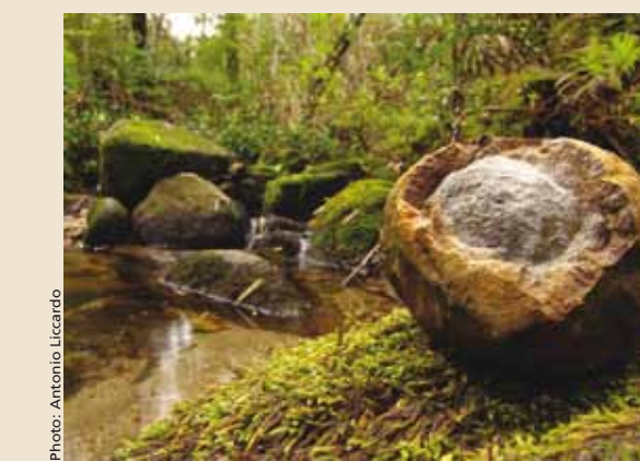
Spheroidal exfoliation of diabase
