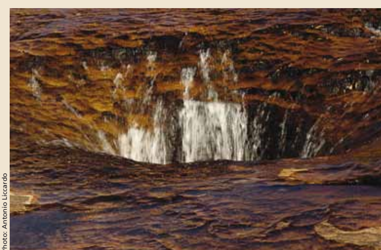
Hollow formed by the erosive action of water on sandstone
