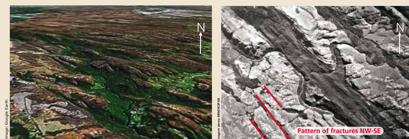
Tridimensional aerial photograph showing the Guartelá Canyon, the general NW-SE trend of the geological structures present, and the different rock types (sandstone walls, volcanic bottom). The bi-dimensional aerial photograph on the right shows the vegetation contrast between these two rock types: dark along the diabase dyke and pale over the less fertile sandstone.
